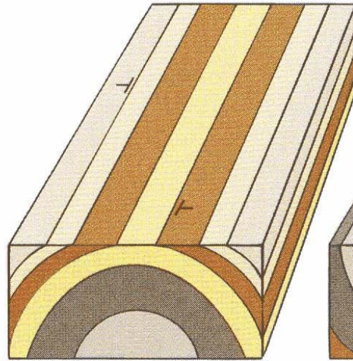
Anticline
