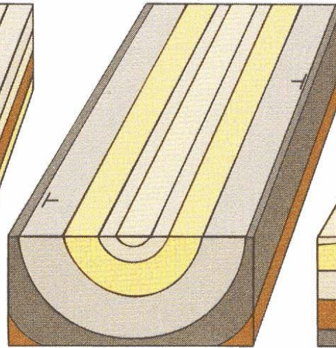
Syncline
